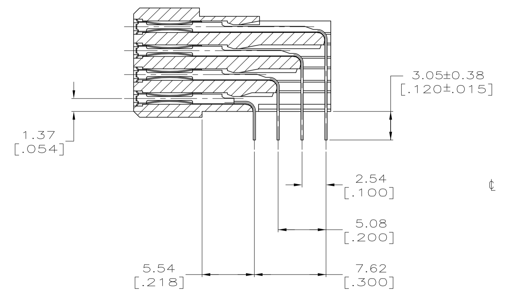
SECTION T-T
